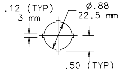
22.5mm 4-WAY
