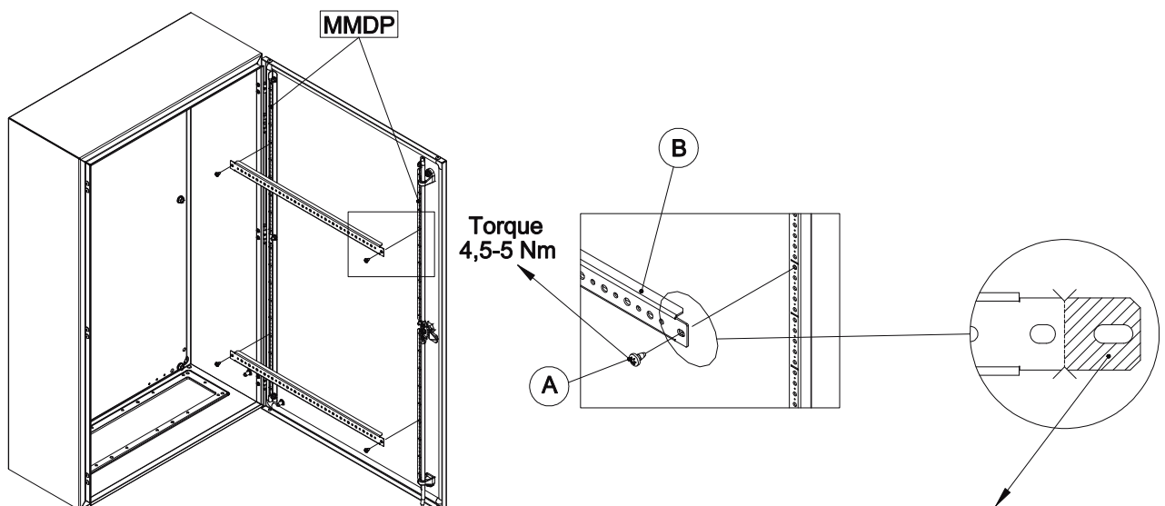
Assembly in enclosures with three point espagnolette locking system
