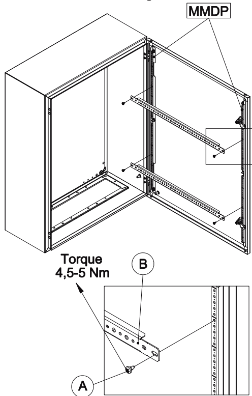
Horizontal mounting
