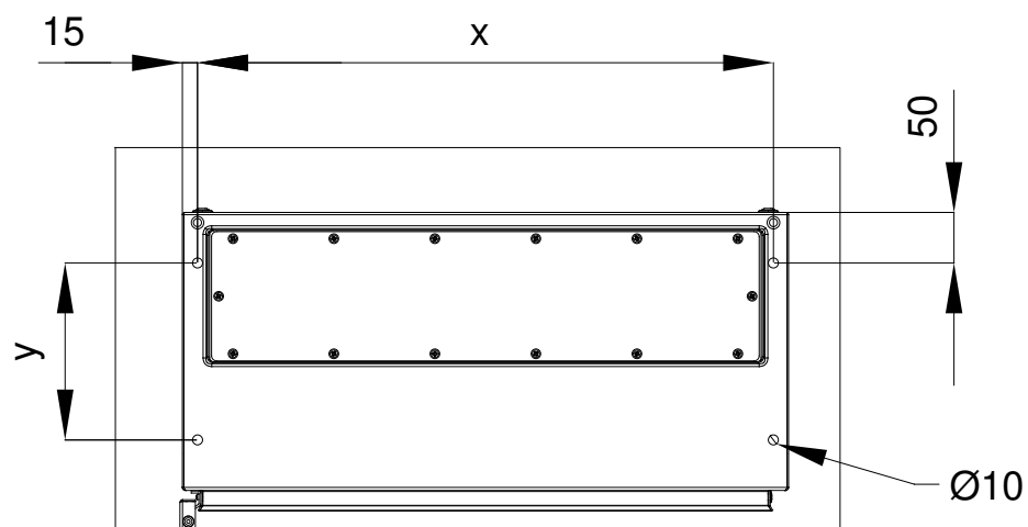
Cut-out dimensions
