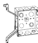
52151DV1/2 DV Bracket provides offset
