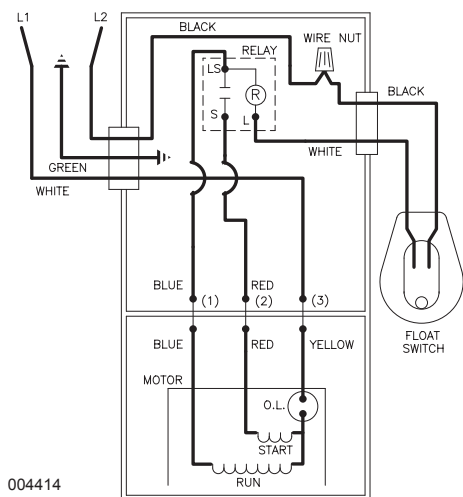
WIRING DIAGRAM FOR MODELS "WM267-C", "WM267-D", and "WM267-E" 10/92 thru Current
