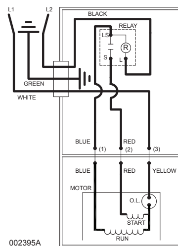
WIRING DIAGRAM FOR MODELS "N267-F", "E267-F", and "I267-F" 10/92 thru Current
