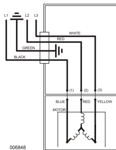
WIRING DIAGRAM FOR MODELS "J267-F", "F267-F" and "G267-F" 10/92 thru Current
