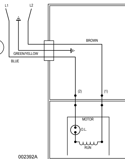
WIRING DIAGRAM FOR MODELS "N53-A", "N53-B" and "N53-C" "E53-A", "E53-B", and "E53-C" 9/81 (VM) thru Current
