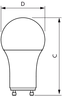
8.8A19/PER/930/P/GU24/DIM 6/1FB T20
