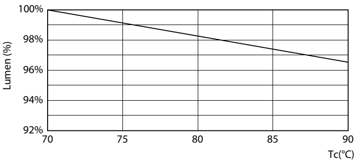
LEDtube_PLCT_11W_30K_LumenVsTc-LMP
