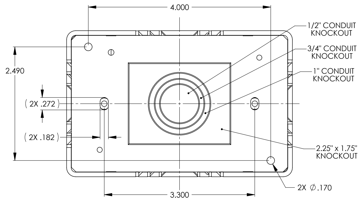
BOTTOM VIEW SHOWN WITHOUT ADHESIVE TAPE
