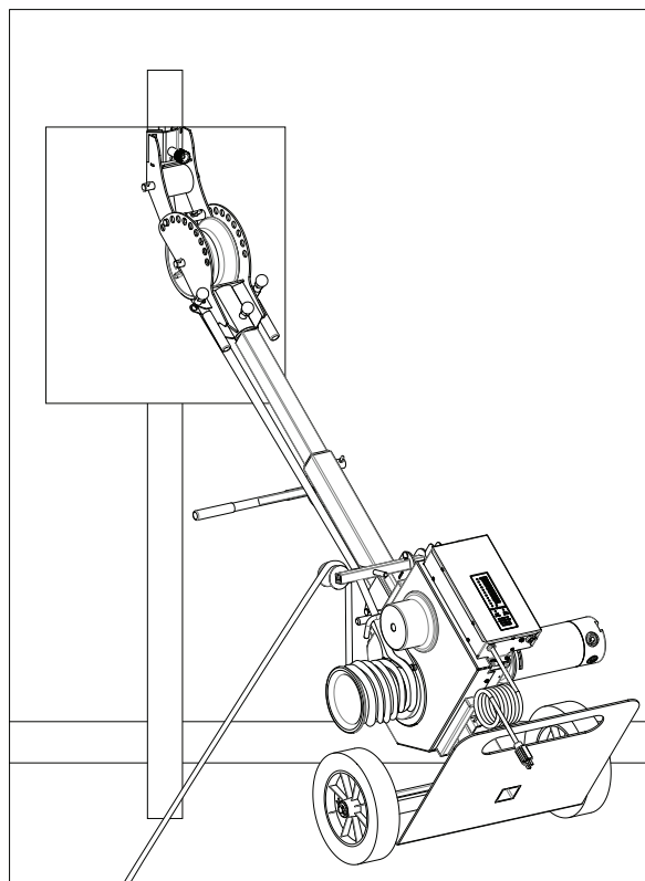
Typical Setup for a Down Pull
