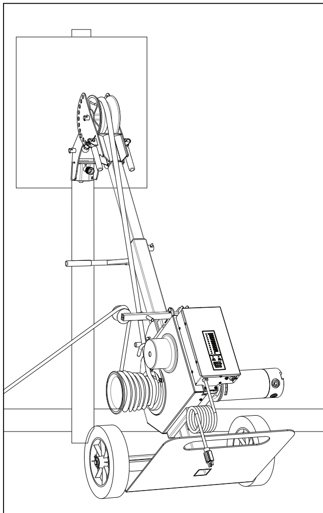
Typical Setup for an Up Pull
