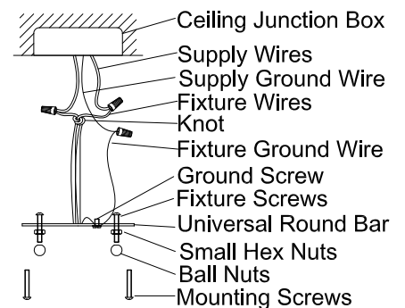
Wiring Drawing (2)
