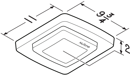
Dimensions shown in inches. Compatible with existing fan housing dimension of 7½" x 7¼" and 8¼" x 8". See chart above for specific models.
