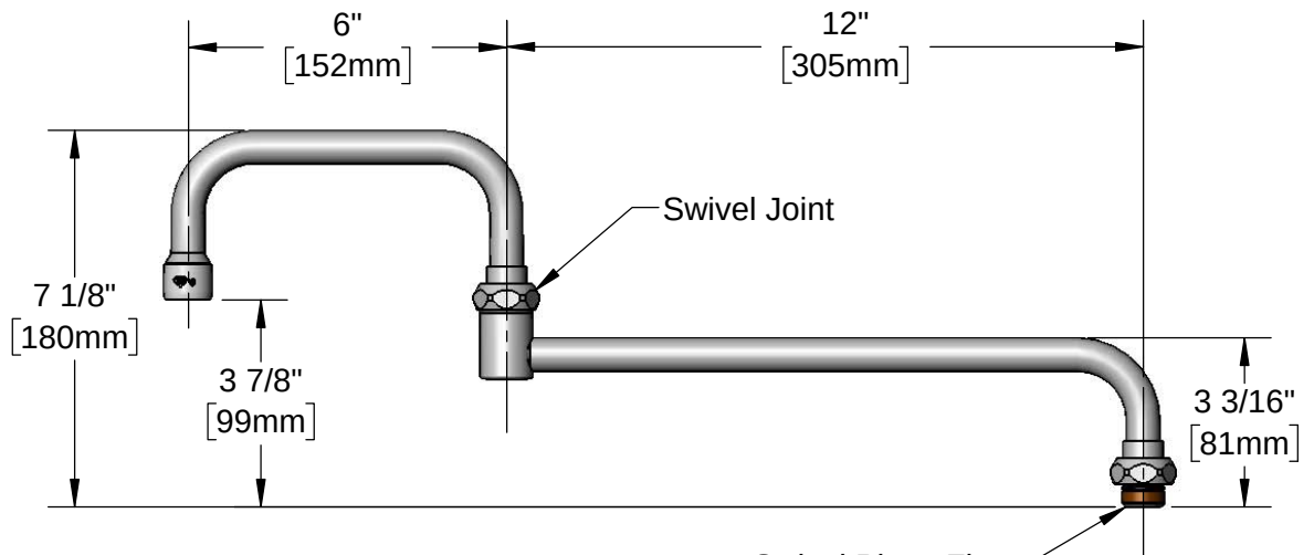
B-PT Stream Regulator Outlet
