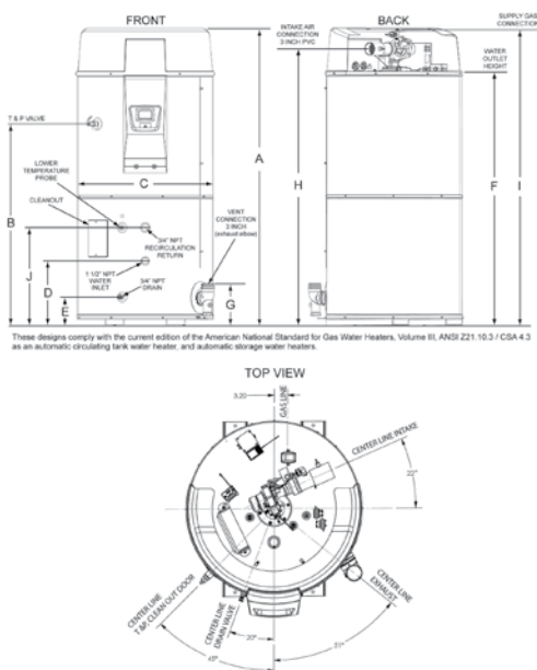
Figure 5. Rough-In Dimensions
