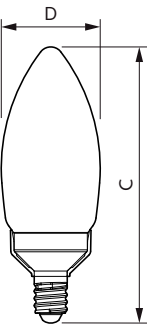
Candle B11 120V 4.5-40W 300lm 2200-2700K
