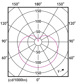
LEDBulb A19 E26 8.8-60W
