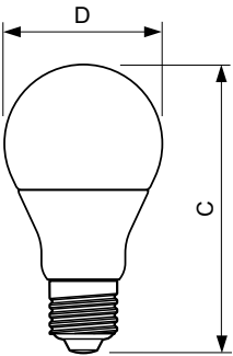
Bulb A19 8.8-60W 800lm 2200-2700K E26 D
