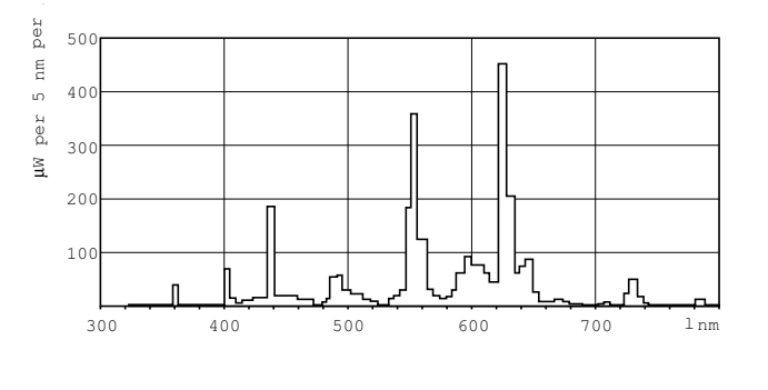
LDPB_TL5-C8_830-Spectral power distribution B/W
