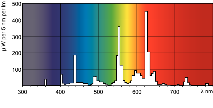
LDPO_TL5-C8_830-Spectral power distribution Colour
