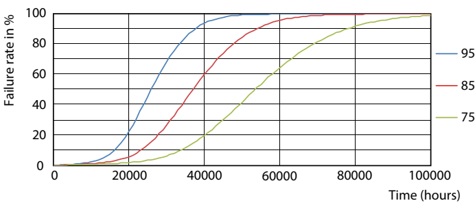
LEDtube G5 25W FailureRate
