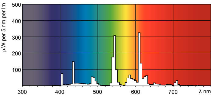
LDPO_PLTTOP4P_835-Spectral power distribution Colour
