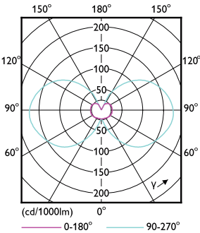
LEDcapsule CorePro 1.7-20W GY6.35 Capsule 827 ND
