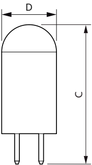
Capsule 12V 2W-20W 200lm 3000K GY6.35 ND
