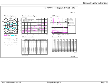
LEDcapsule CorePro 1.7-20W GY6.35 Capsule 830 ND
