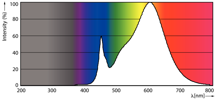
G13 4000K 1400lm
