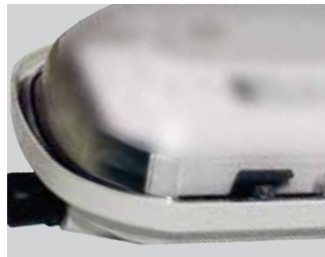
Latch assembly and elastomer gasket seals against water and dust ingress (IP66)
