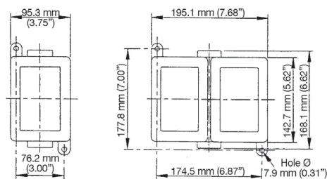
Mounting Box
