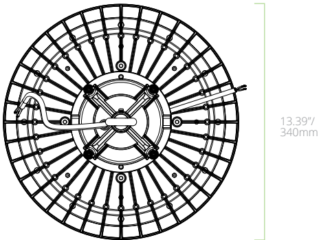
BAYE2/240W (WITH 6' POWER CORD)
