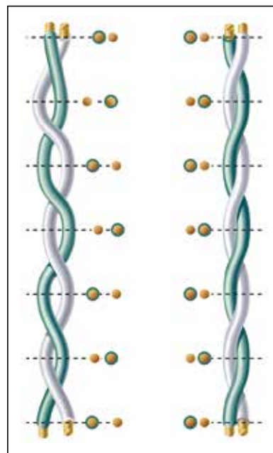
Illustration 3: Side-by-side comparison. Non-Bonded-Pair versus Bonded-Pair cable.
