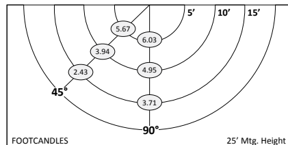
90W Full Cutoff Wall Pack Footcandles On The Ground
