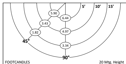
70W Full Cutoff Wall Pack Footcandles On The Ground
