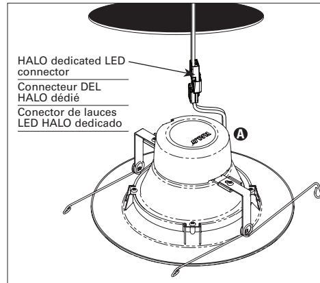
Figure 2. LED Connection
