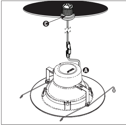
Figure 1. Retrofit Connection
