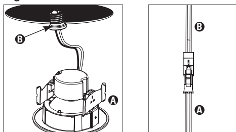
Figure 5. Retrofit Connection
