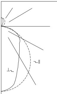
I8-332-UNV-EB81-UPL Electronic Ballast F32T8/TL835 Lamps 3000 lumens Spacing criterion: (H) 1.2 x mounting height, (L) 1.1 x mounting height Efficiency 94.1% Test Report: I8-332-UNV-EB81-UPL.IES
