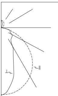
IS-354T5-UNV-EBT2-UPL (2) Electronic Ballasts (3) F54T5/HO/830K lamps 4400 lumens Spacing criterion: (H) 1.2 x mounting height, (L) 0.7 x mounting height Efficiency 98.2% Test Report: IS-354T5-UNV-EBT2-UPL.IES
