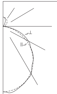
I8-432-UNV-EB81-UPL Electronic Ballast F32T8-TL835 lamps 3000 lumens Spacing criterion: (H) 1.2 x mounting height, (L) 1.3 x mounting height Efficiency 91.2% Test Report: I8-432-UNV-EB81-UPL.IES
