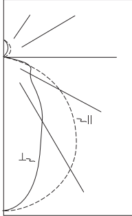
IS-454T5-UNV-EBT2-UPL (2) Electronic Ballasts (4) 54W T5 lamps 4400 lumens Spacing criterion: (H) 1.2 x mounting height, (L) 0.8 x mounting height Efficiency 92.8% Test Report: IS-454T5-UNV-EBT2-UPL.IES
