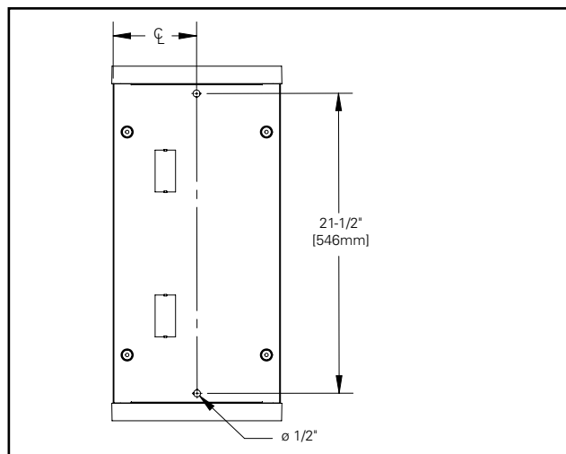
Diagram 3: Pendant Mounting
