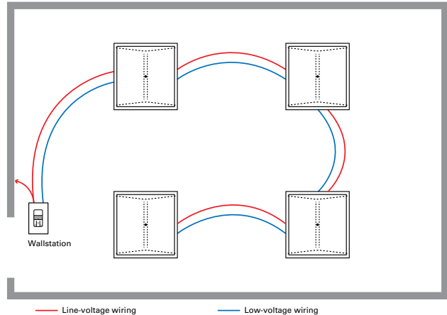
0-10V Dimming & Sensing
