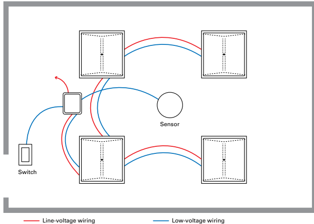
Typical 0-10V Dimming & Sensing
