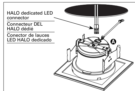
Figure 7. LED Connection
