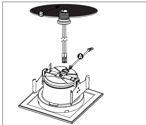
Figure 5. Retrofit Connection
