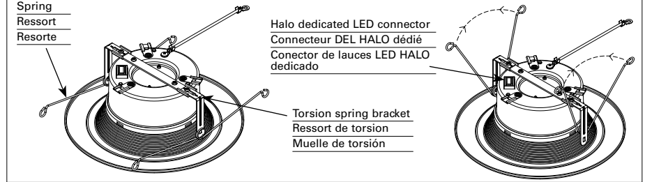
Figure 7. LED Connection
