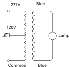
Wiring Diagram (H36LVTAT277 ONLY)
