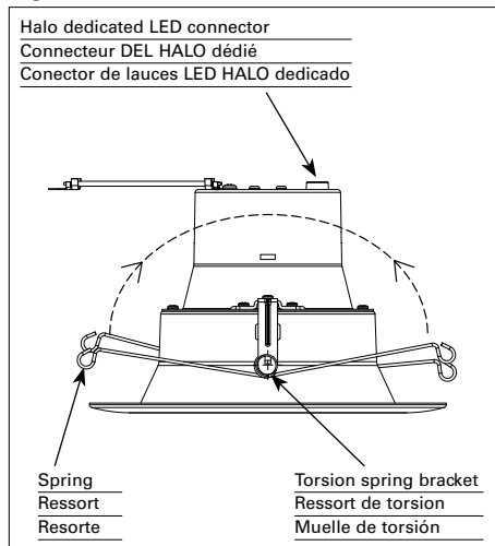
Figure 7. LED Connection
