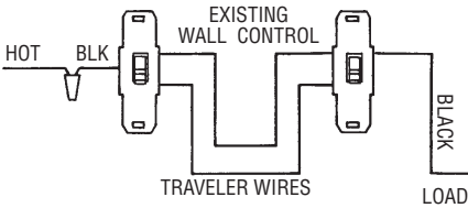
3-WAY WIRING DIAGRAM: RETROFIT
