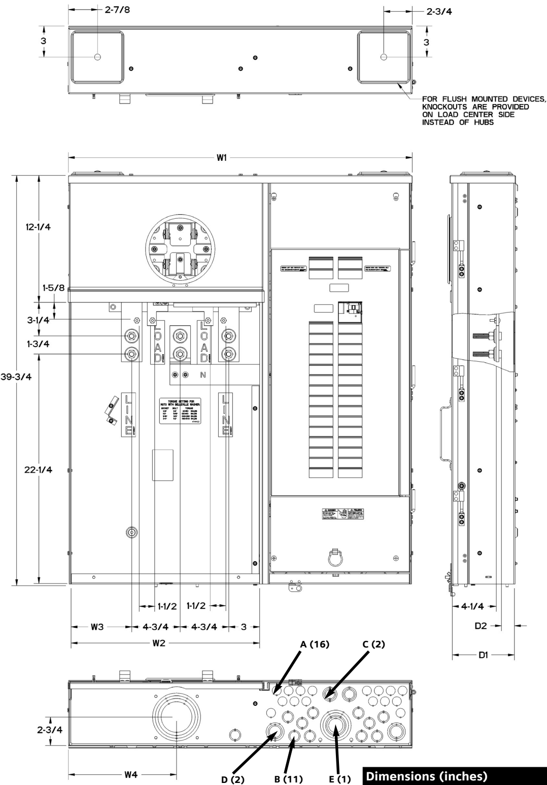
Diagram MC3042B1400SCS
