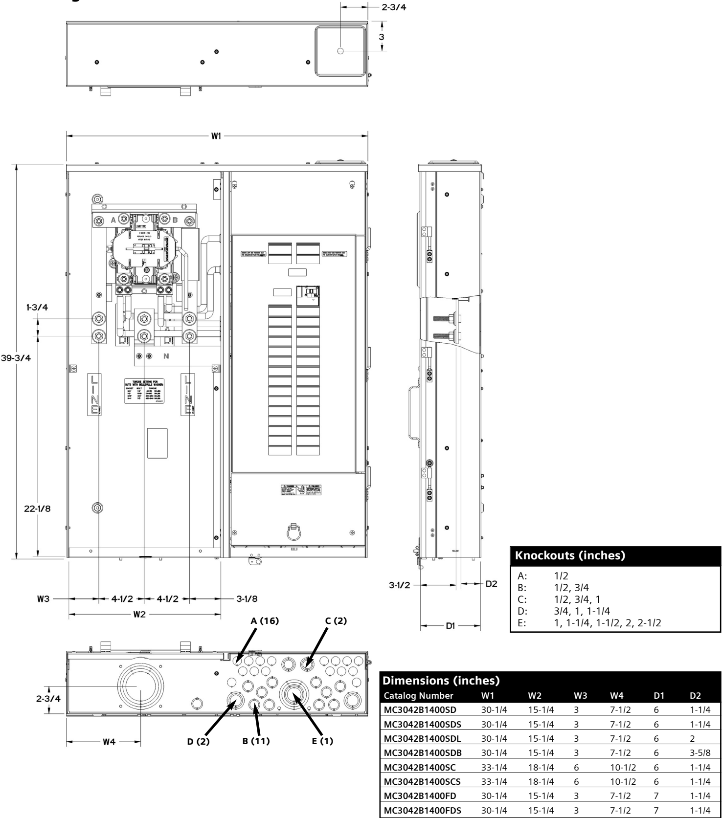
Diagram MC3042B1400SDL
