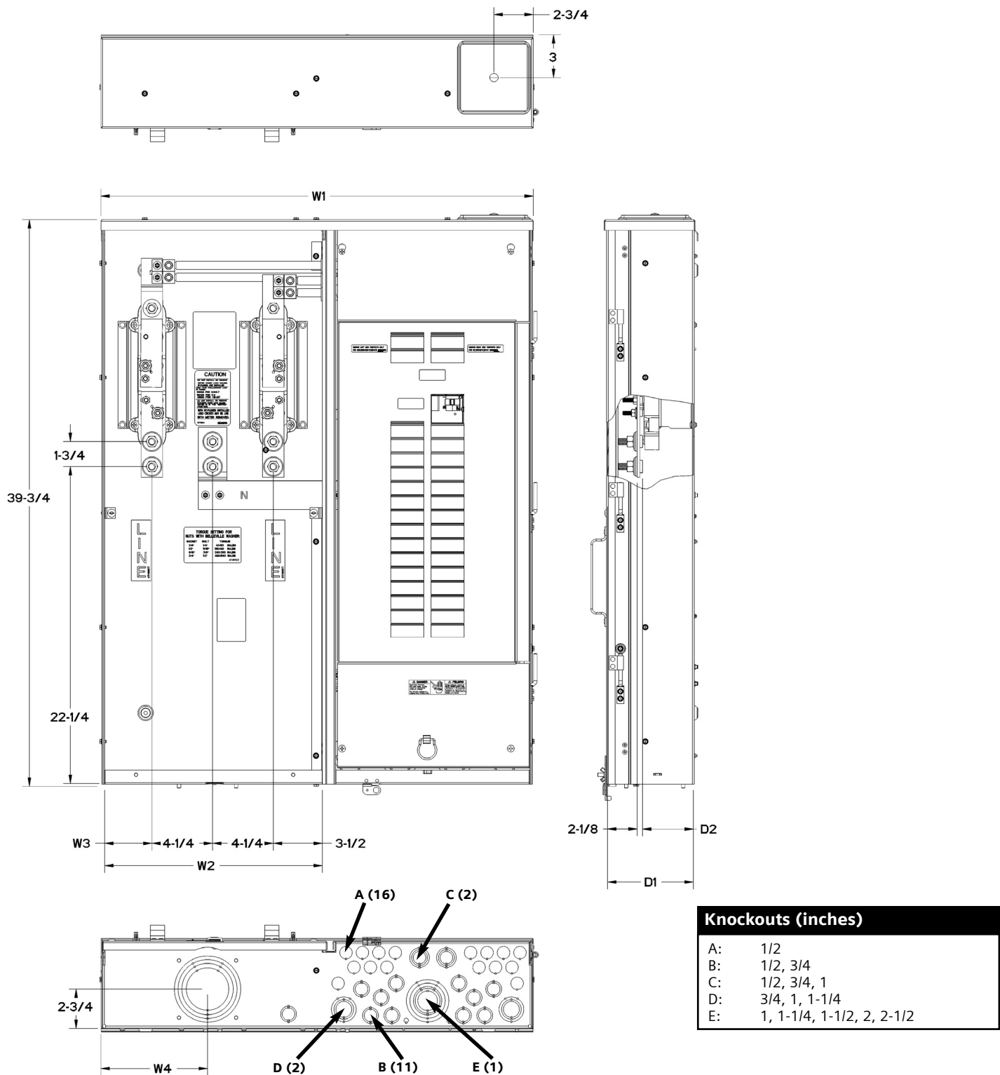
Diagram MC3042B1400SDB
