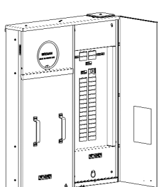
Plug-in, Underground Feed, Surface Mount
