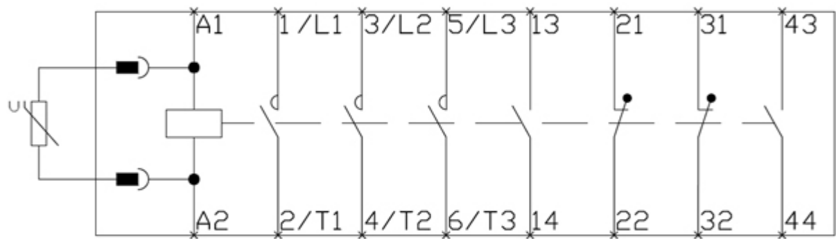
LENO0F G & H Wiring Diagram
