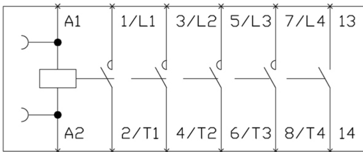
LEN00B004 Wiring Diagram
