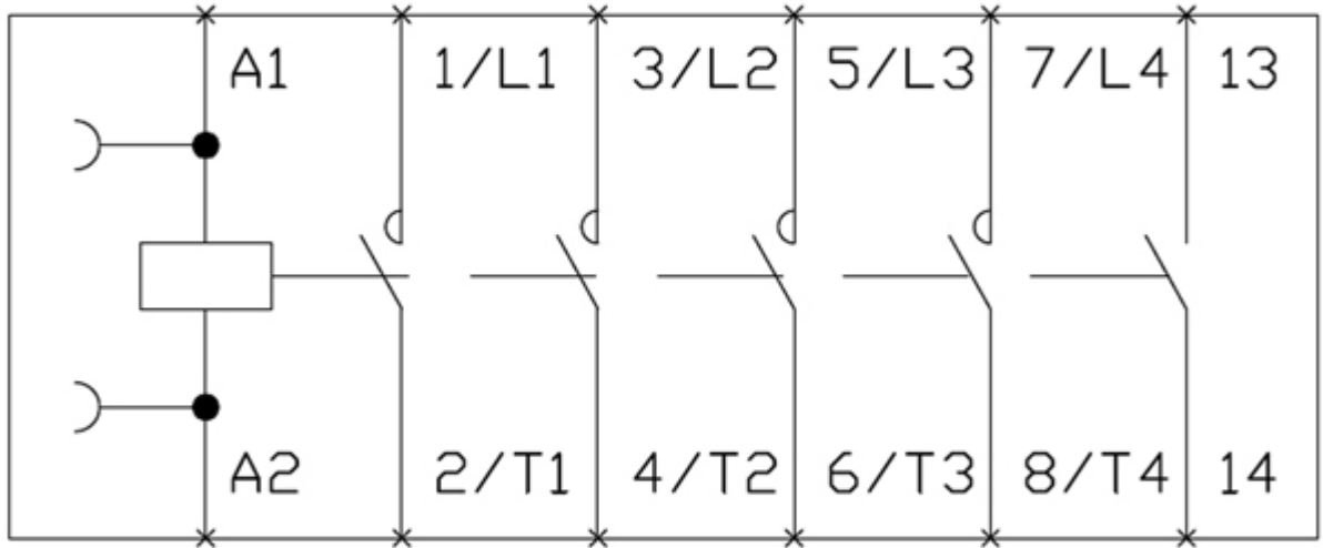
LENO0B004 Wiring Diagram
