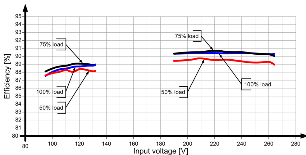
Figure 6-21 6EP1337-3BA00 efficiency
