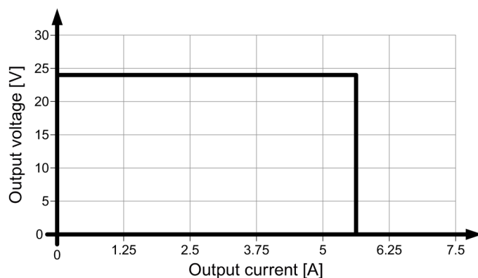
Figure 6-3 6EP1333-3BA10 single operation output characteristic
