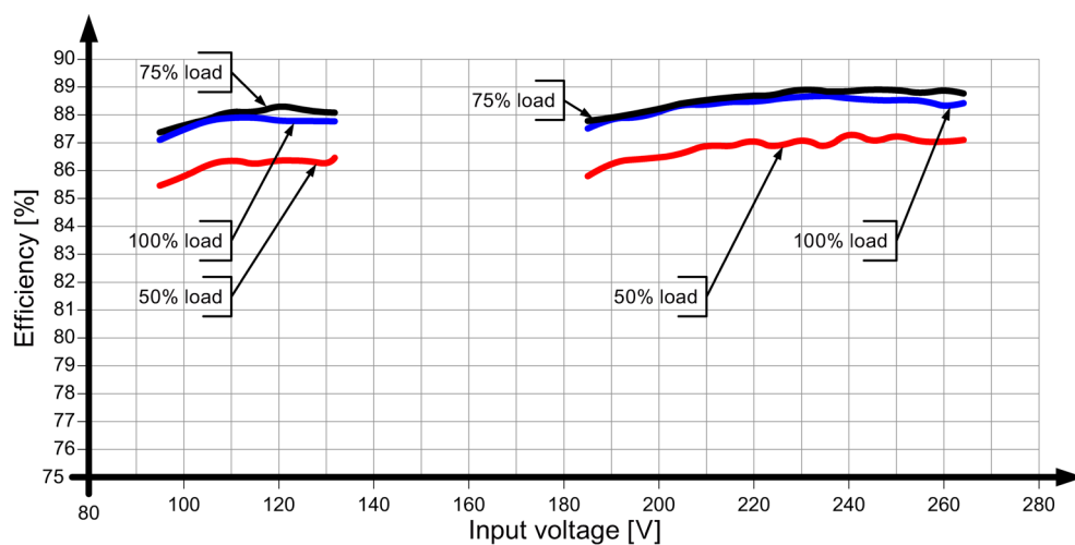
Figure 6-20 6EP1336-3BA00 efficiency
