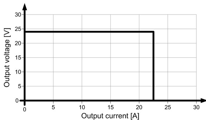
Figure 6-5 6EP1336-3BA00 single operation output characteristic
