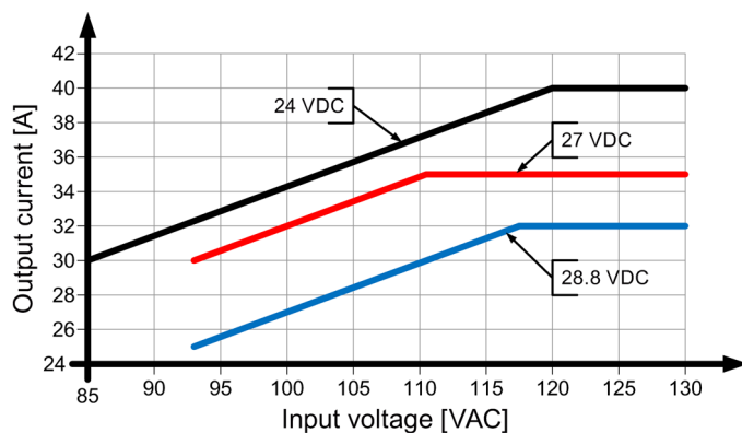
Figure 6-9 Output derating depending on the input voltage
