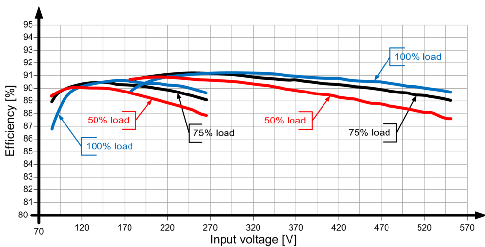
Figure 6-19 6EP1334-3BA10 efficiency
