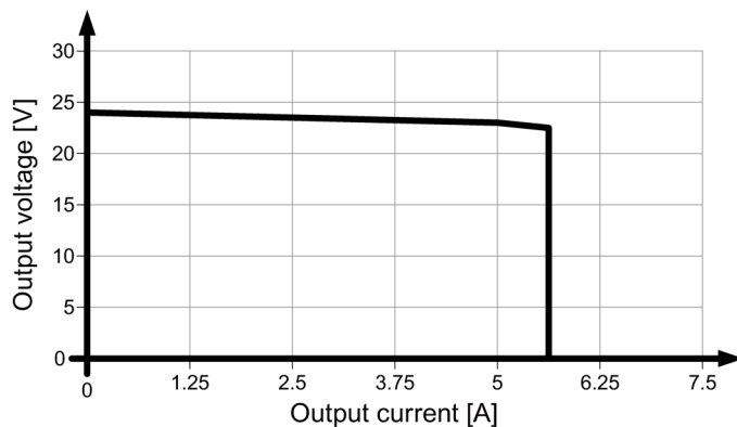
Figure 6-10 6EP1333-3BA10 parallel operation output characteristic
