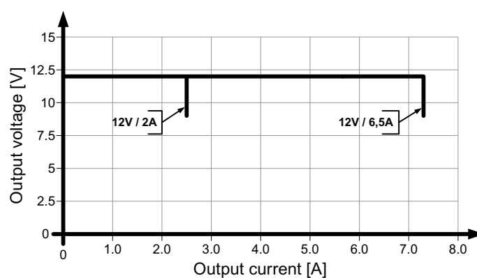
Figure 6-3 12 V output characteristic
