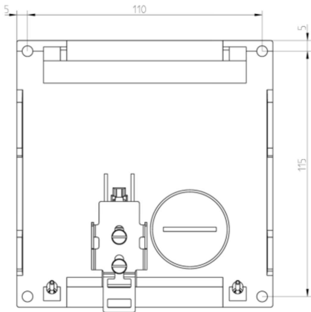
Image A-2 Drilling pattern SCALANCE X212-2, X212-2LD and X216
