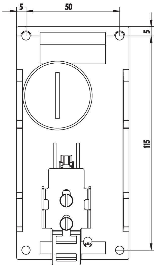
Image A-1 Drilling pattern SCALANCE X204-2, X204-2TS, X204-2FM, X204-2LD, X204-2LD TS, X206-1, X206-1LD, X208, X200-4P IRT, X201-3P IRT, X202-2IRT, X202-2P IRT, X204IRT
