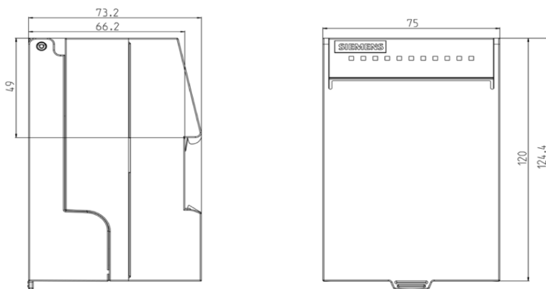
Image A-8 SCALANCE XF-200 dimension drawings
