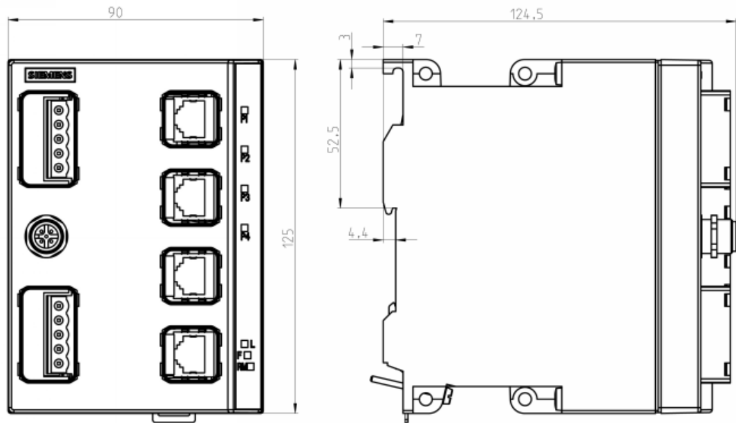
Image A-6 Dimension drawings of the SCALANCE X208PRO, SCALANCE X201-3P IRT PRO, SCALANCE X202-2P IRT PRO and SCALANCE X204IRT PRO
