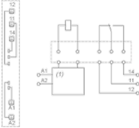
(1) Protection circuit
