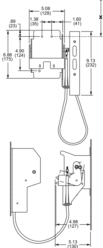
9422CSF 3-Pole
