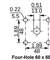
Four-Hole 60 x 60 Mounting Dimensions [9]
