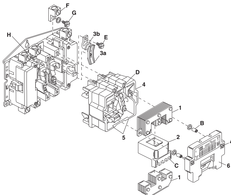
Figure / Figura / Figure 1 : Assembly / Ensamble / Assemblage
