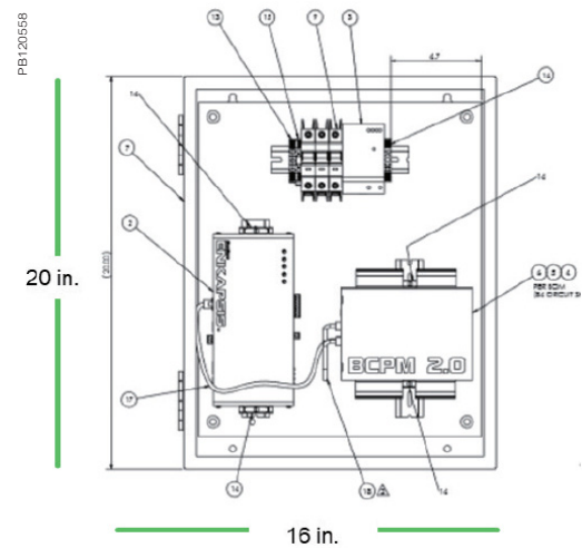
PowerLogic™ HDPM6000 medium size enclosure
