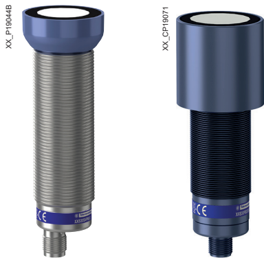
XXS30S4PM12 XXS30P8M12
