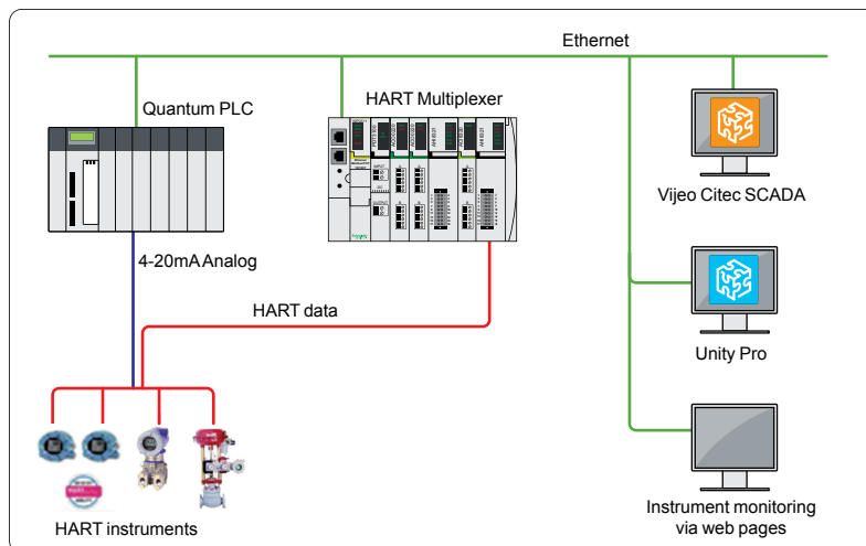
HART multiplexer and devices in a global automation architecture
