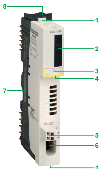
EOS/BOS internal bus expansion modules STBXBE100K
