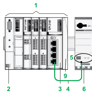
TeSys U connected to a standard Modicon STB
