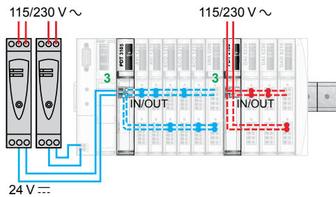
Configuration with basic PDM and two separate 24 V power supplies
