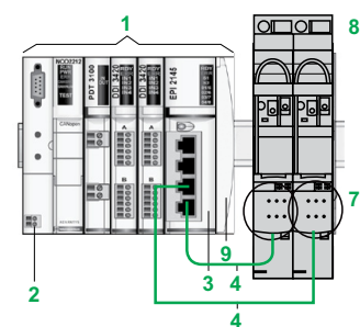
Reversing TeSys Quickfit connected to a standard Modicon STB
