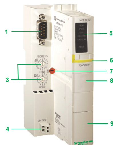
STBNCO2212 CANOpen bus interface module
