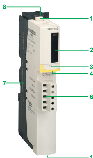
CANopen expansion module STBXBE2100K
