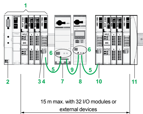
TeSys U as preferred module on a standard Modicon STB
