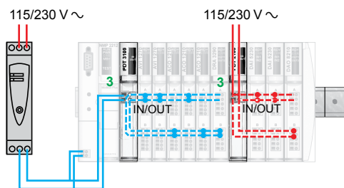
Configuration with basic PDM and one 24 V power supply
