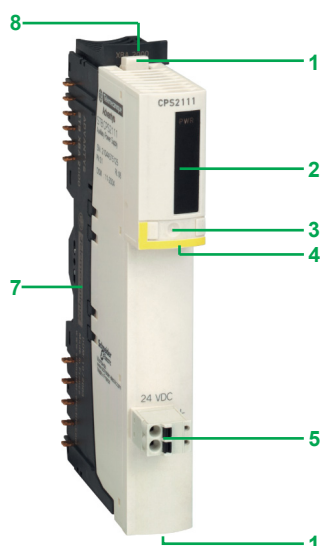
Auxiliary power supply module STBCPS2111K
