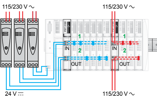
Configuration with standard PDM and three separate 24 V power supplies
