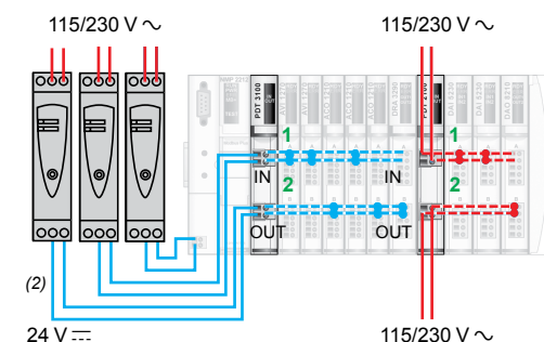
Configuration with standard PDM and three separate 24 V DC power supplies
