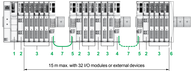
Standard Modicon STB with 3 segments
