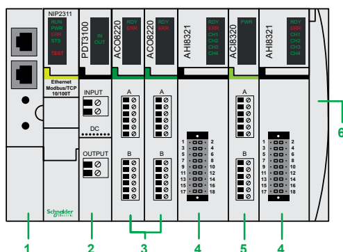
Example of an 8 HART channels solution
