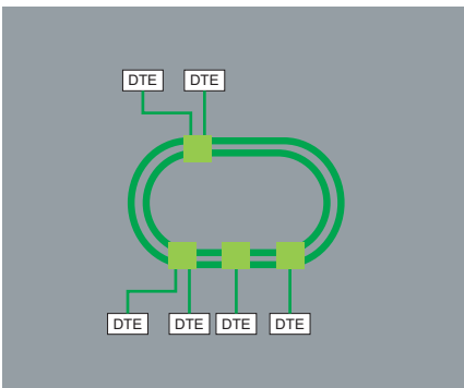
Dual ring topology
