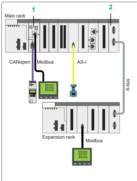
Integrated fieldbus architecture
