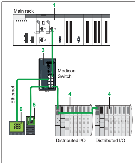
4 Distributed I/O architecture: devices distributed over Ethernet with BMXNOE0110 module and Modicon Switch
