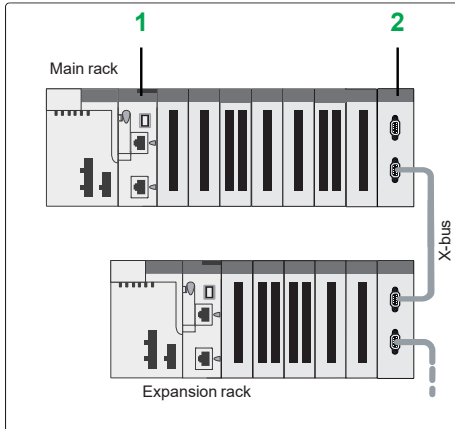
Local I/O architecture
